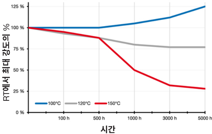
Heat aging
