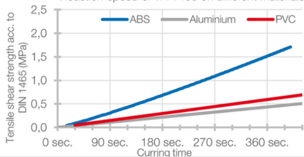
Reaction speed of VA 1408 on different materials
