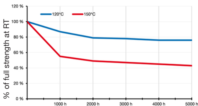
Heat aging
